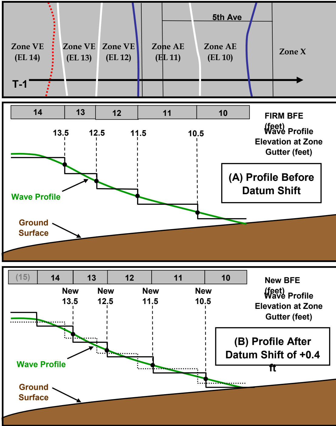
Figure 22: Comparison of gutter locations prior to a datum conversion (A) and after (B). Although Zone VE (EL 15) can be identified on the new wave profile, it lies seaward of the mapped shoreline position and thus may not need to be included on the FIRM.
