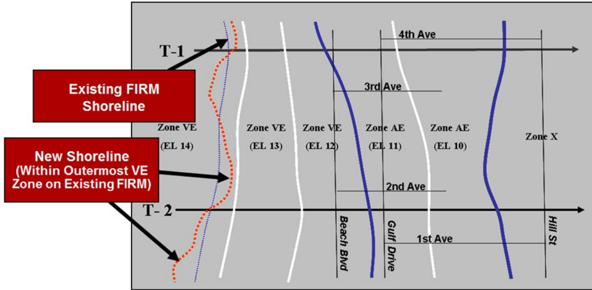
Figure 20: Work map depicting the flood zones, BFEs, and shoreline from the effective FIRM and the new shoreline position (modified from DiCamillo et al., 2005). T-1 and T-2 represent transect locations. Because the shoreline retreat is restricted to the outermost VE Zone (EL 14), it has no impact on remapping of flood zones.
