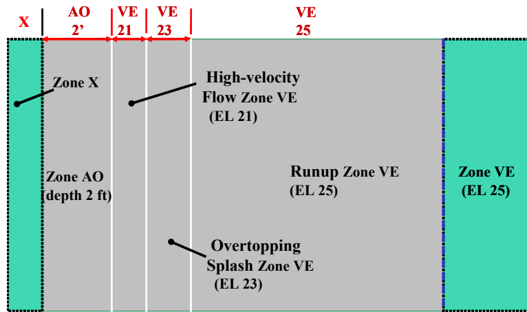
Figure 9: Erodible Low Coastal Bluff with VE Zone Controlled by Wave Runup, Overtopping Splash, and High-velocity Flow
