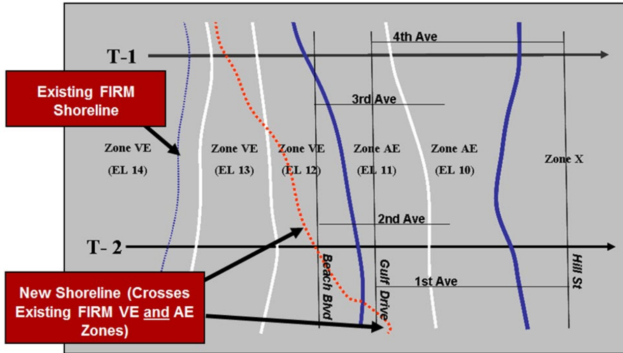
Figure 23: Work map depicting existing shoreline position from the effective FIRM and the new shoreline location (modified from DiCamillo et al., 2005). Because the shoreline retreat extends landward of the effective VE/AE boundary, reanalysis of flood hazards may be warranted (in lieu of redelineation).
