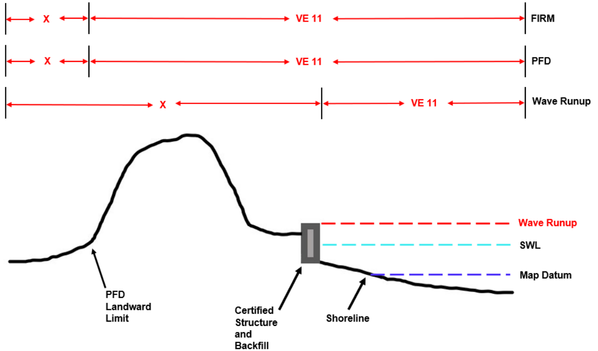
Figure 18: Placement of the Landward Limit of the VE Zone in an Area with a Certified Coastal Protection Structure Seaward of the PFD.
