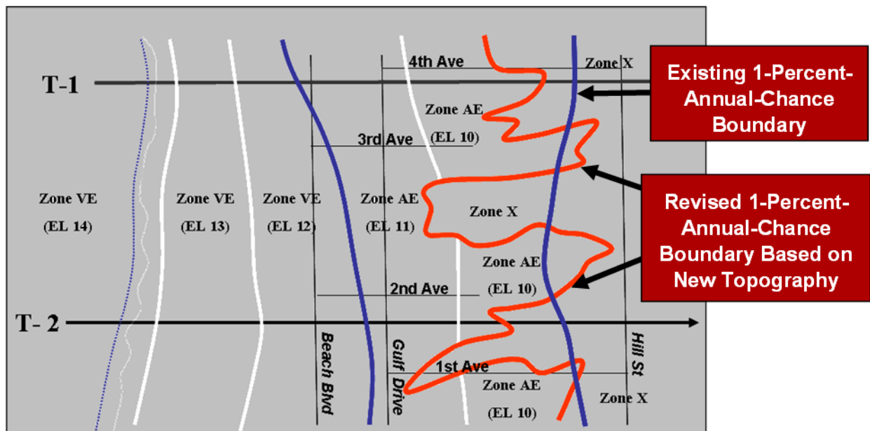
Figure 21: Work map depicting the existing 1-percent-annual-chance floodplain boundary from the effective FIRM, and the new boundary redelineated based on the effective SWEL and new topographic data (modified from DiCamillo et al., 2005).
