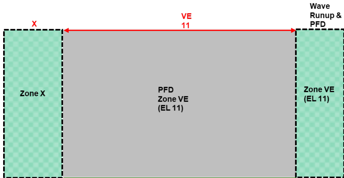
Figure 19: Placement of the Landward Limit of the VE Zone in an Area with a Certified Coastal Protection Structure Seaward of the PFD.
