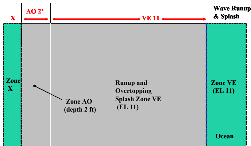
Figure 12: Sandy Beach Backed by Low Sand Dune with Overtopping Splash Controlling VE Zone
